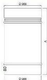
Easy-Line Extension piece 330 mm, Ø300 mm Stainless steel
