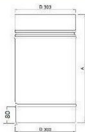
Easy-Line Extension piece 1000 mm, Ø300 mm Stainless steel
