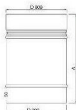
Easy-Line Extension piece 200 mm, Ø300 mm Stainless steel
